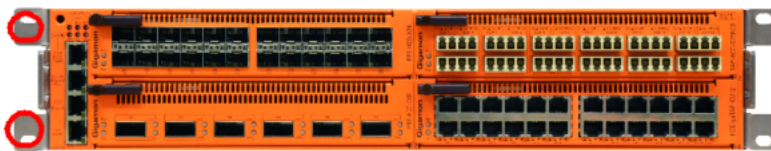
Cable Management Assembly Attached The screws attach from the inside of the tabs. You may need to partially remove the modules in bays 1 and 4 to fully attach the cable management assembly screws.
