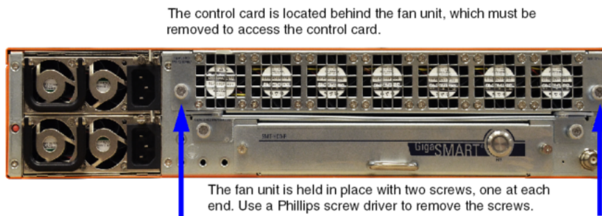
Figure 1 Replacing a Control Card
